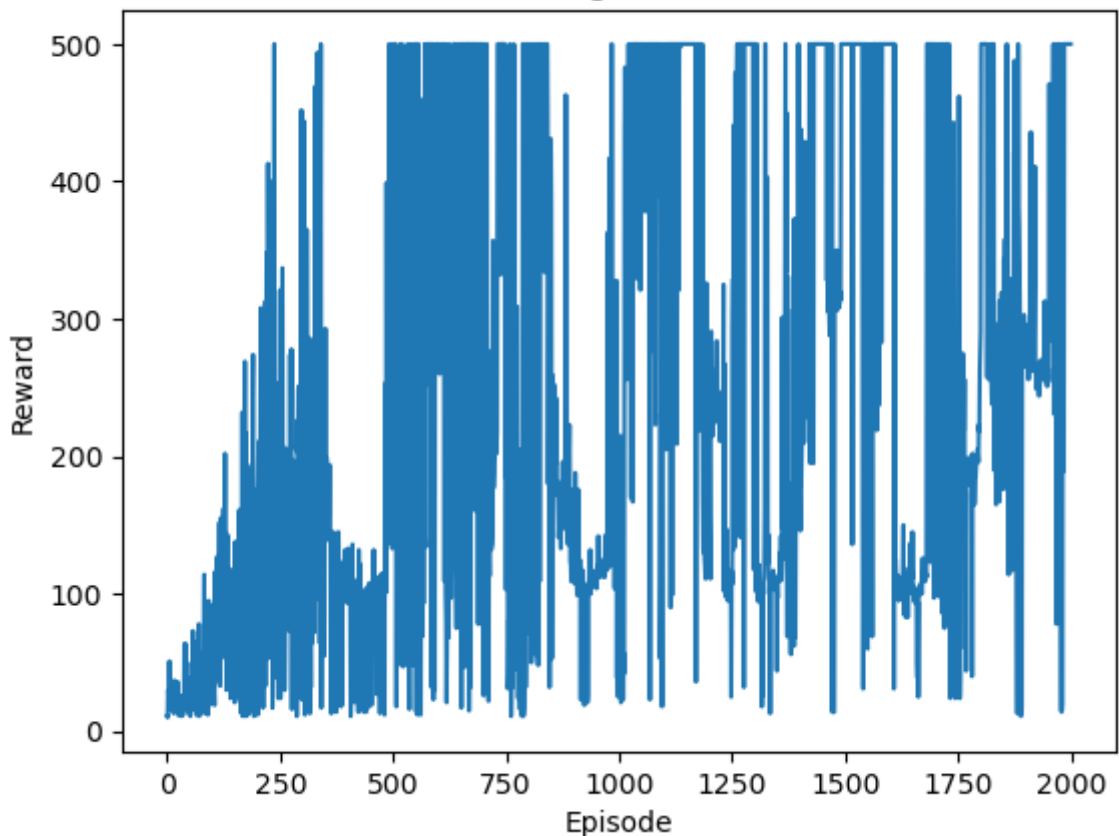
Training Rewards
